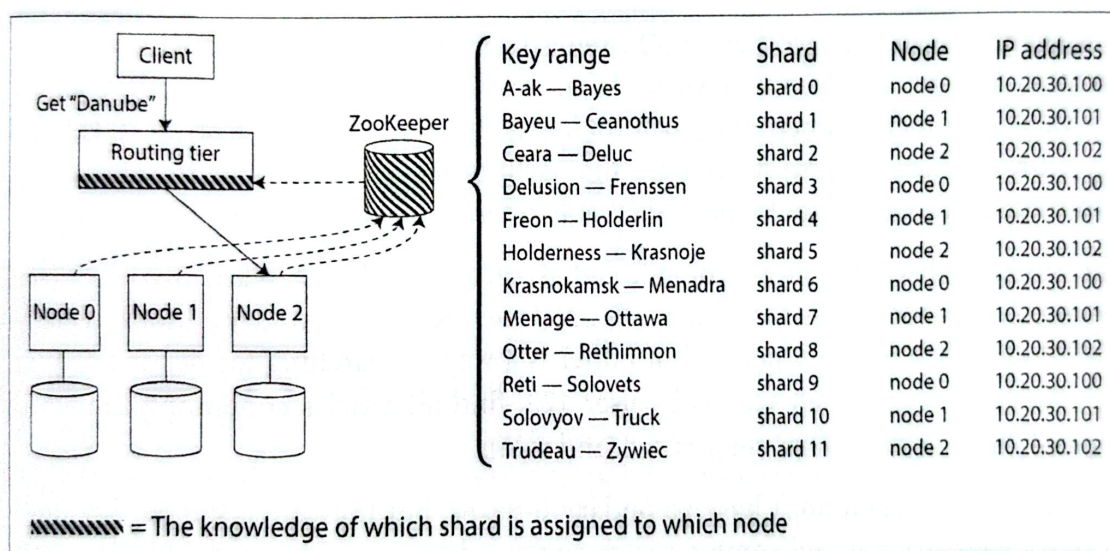
Figure 7-8. Using ZooKeeper to keep track of the assignment of shards to nodes
